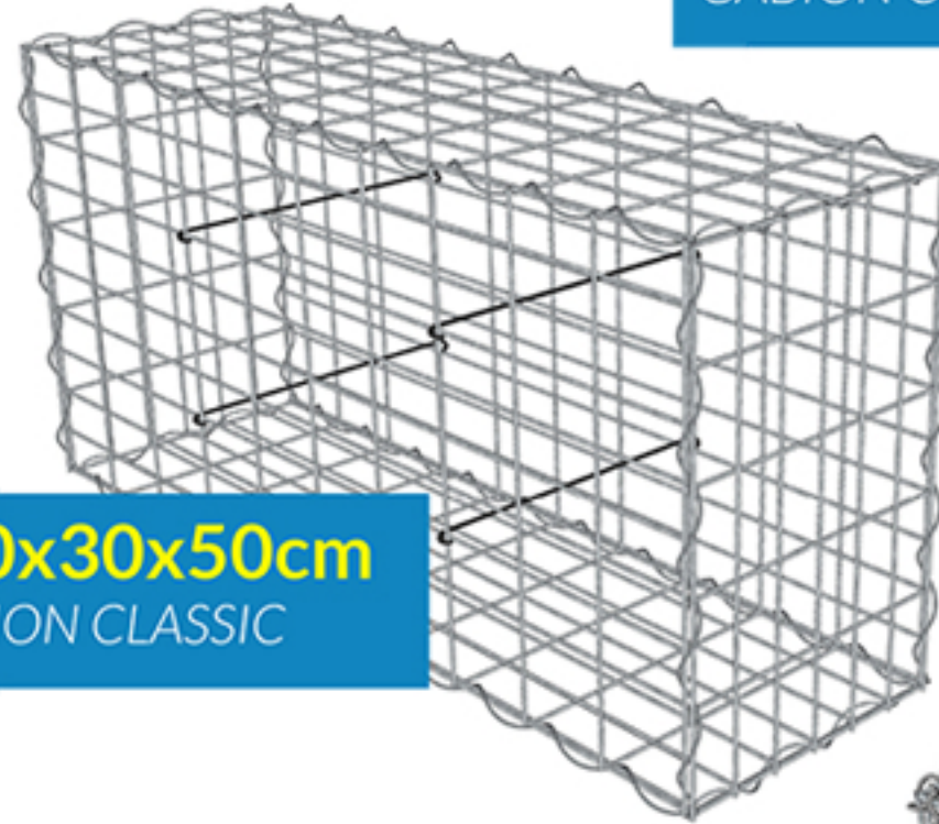
100x50x50cm GABION CLASSIC
